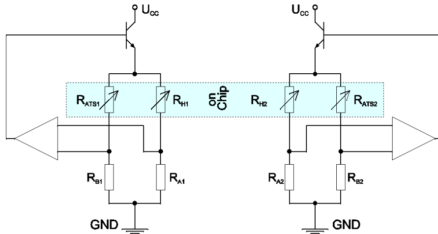
Figure 3: Above is shown an example of a measurement electronics using a Wheatstone-bridge. The resistors R_{Ax} and R_{Bx} need to be trimmed to operate the heater at a defined over-temperature
